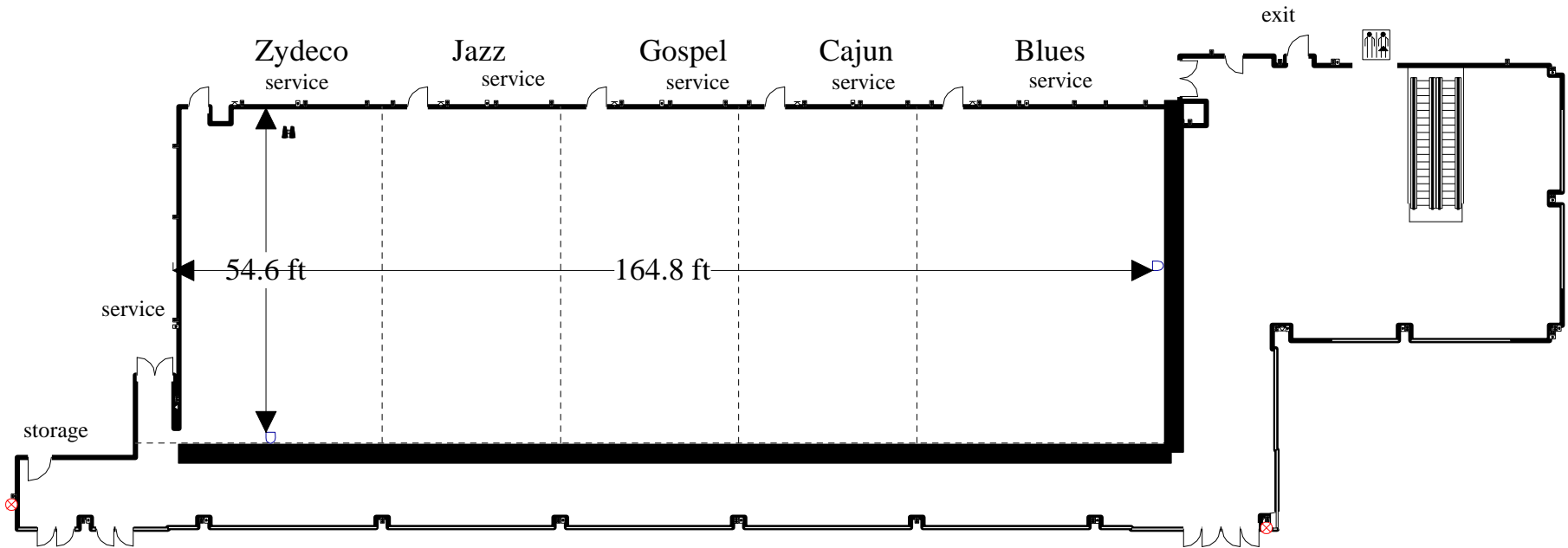
FESTIVAL BALLROOM WITH DIMENSIONS AND ELECTRICAL OUTLETS SHOWN ON WALLS
